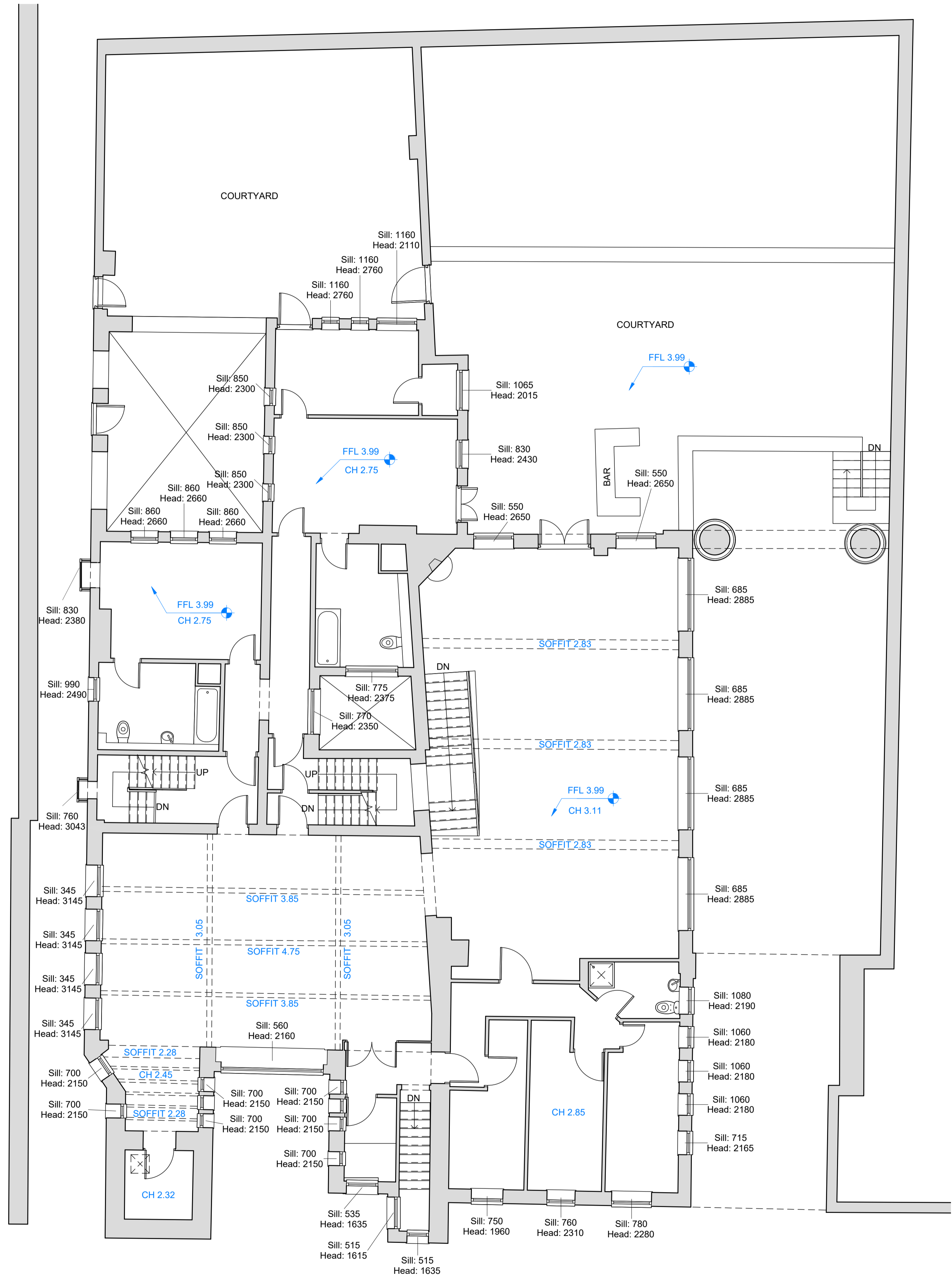
1 First Floor 1 : 75
