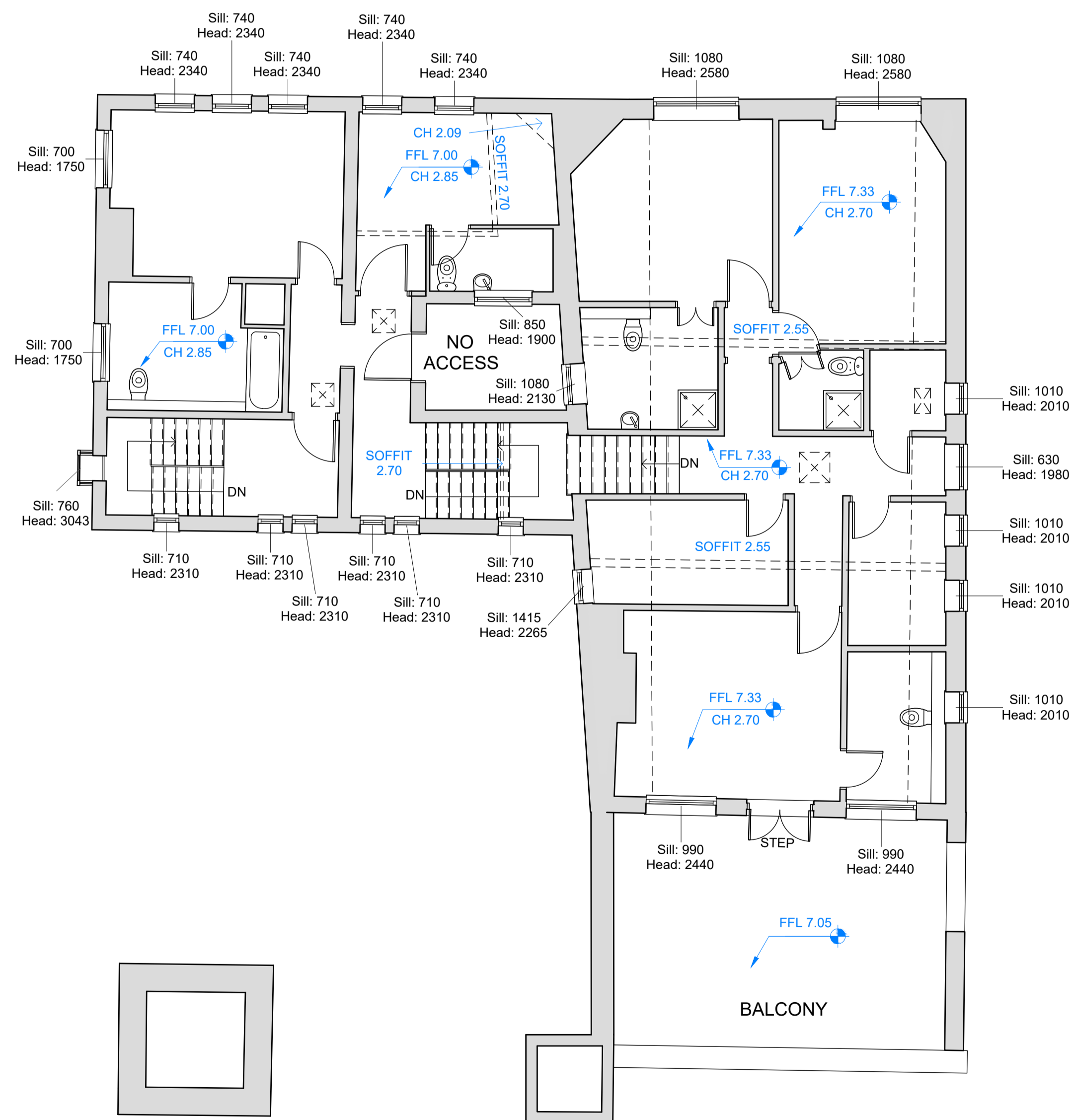
1 Second Floor 1 : 75
